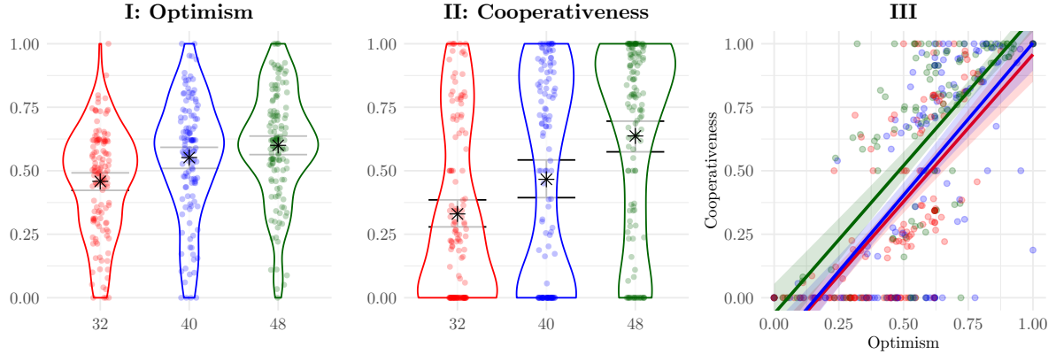
Figure 5: Optimism and cooperativeness in Supergame 1: Violin and scatter plots
