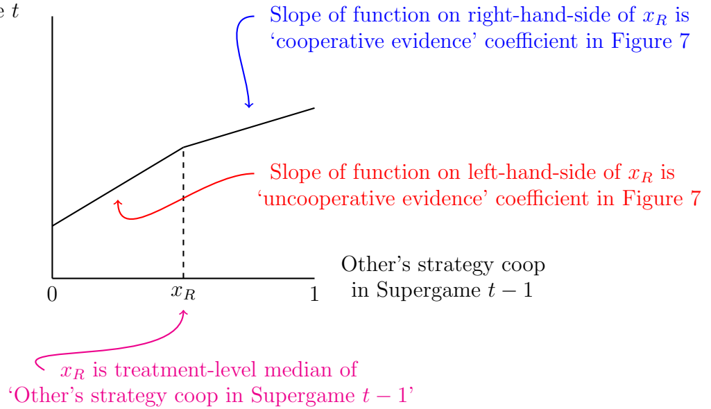
Figure 8: Understanding the coefficients from Figure 7
