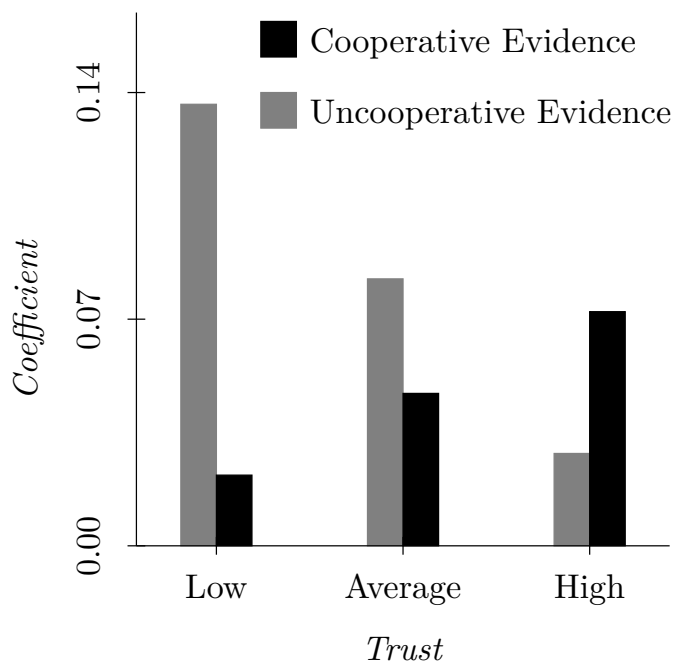
Figure 7: Effect of opponent's strategy cooperation in Supergame t - 1 on strategy cooperation in Supergame t
