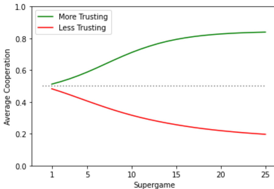
Figure A.24: Simulated dynamics of cooperation in more trusting and less trusting sessions
