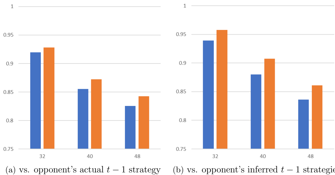
Figure A.20: Payoff of revised strategy at t (orange) and original strategy at t - 1 (blue), playing against opponent's t - 1 strategy (as proportion of payoff from best-response)
