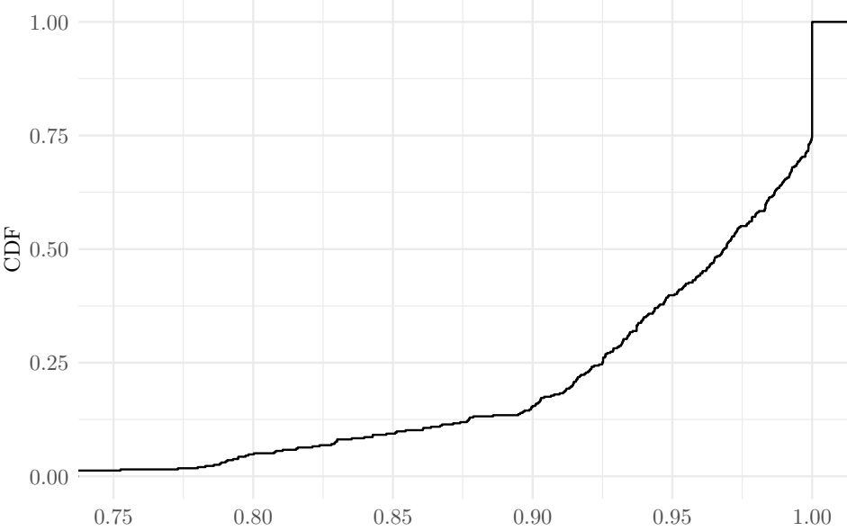
Figure A.27: CDF of payoffs relative to best responding to beliefs in Supergame 1
