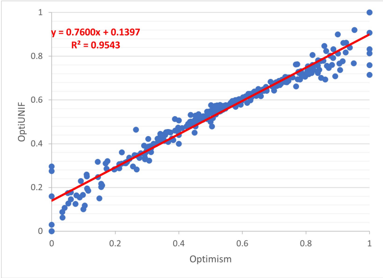
Figure A.28: Scatterplot of optiUNIF vs. optimism in Supergame 1
