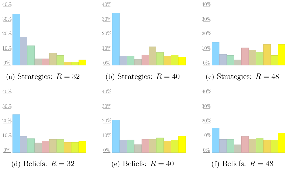
Figure A.21: Strategies & average beliefs in Supergame 1 (replicates Figure 3)
