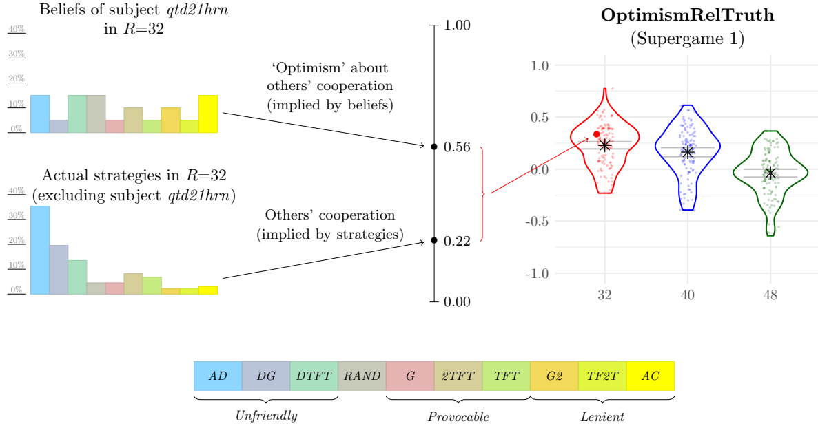
Figure 4: Construction of violin plots of OptimismRelTruth in Supergame 1
