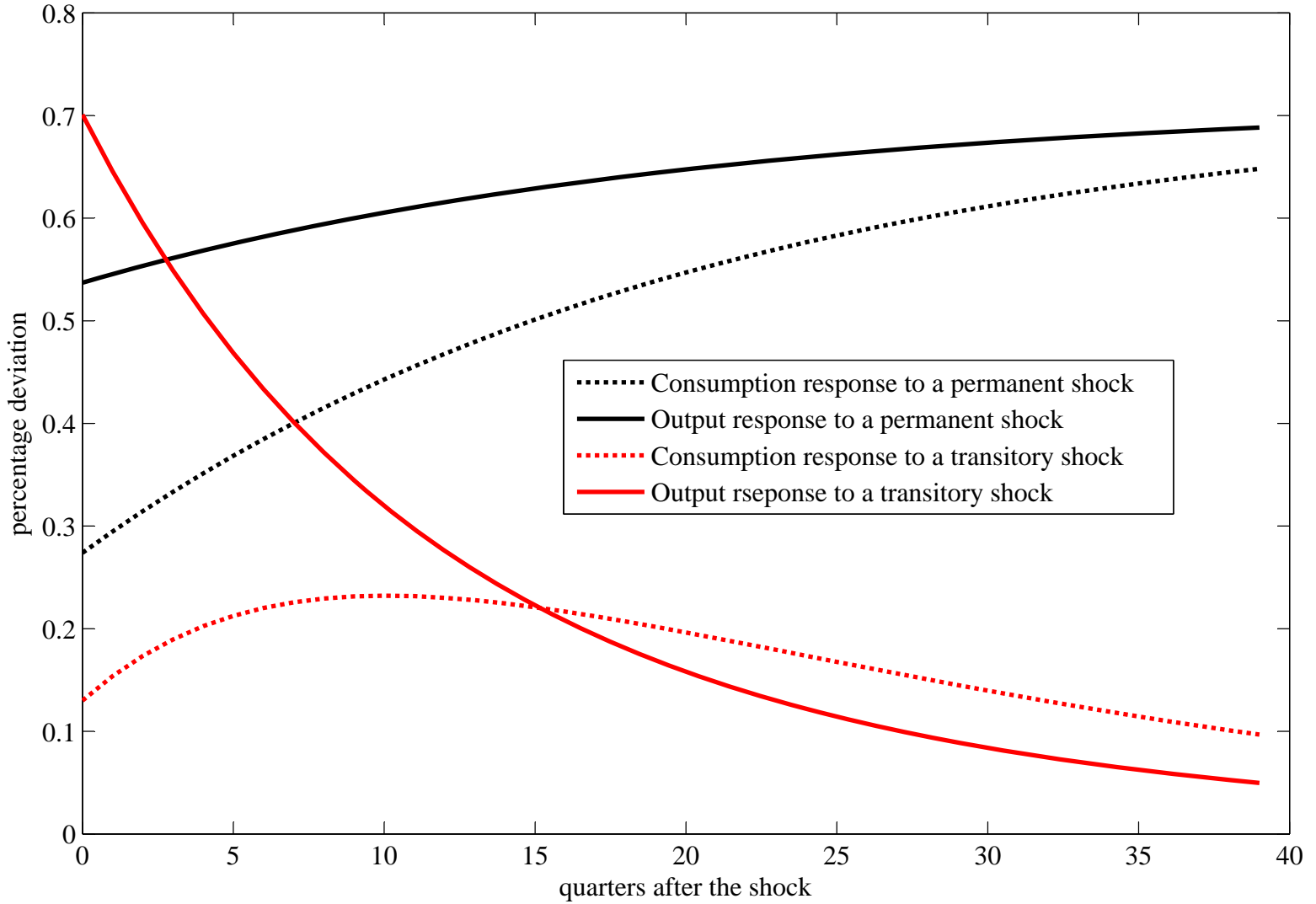
Figure 1. Impulse responses from King, Plosser and Rebelo Model
